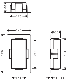
XtraStoris Minimalistic 300 x 150 x 100 mm
