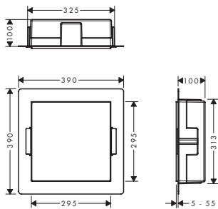
XtraStoris Minimalistic 300 x 300 x 100 mm
