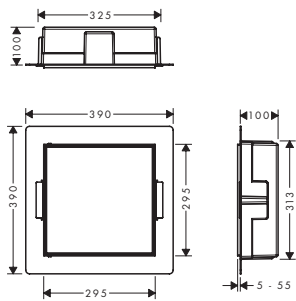
XtraStoris Rock 300 x 300 x 100 mm
